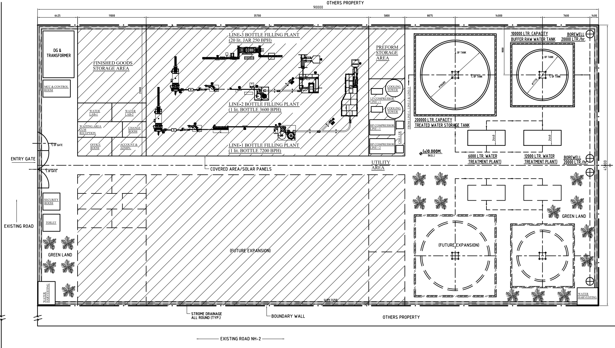
LAYOUT PLAN (SCALE 1:130)
